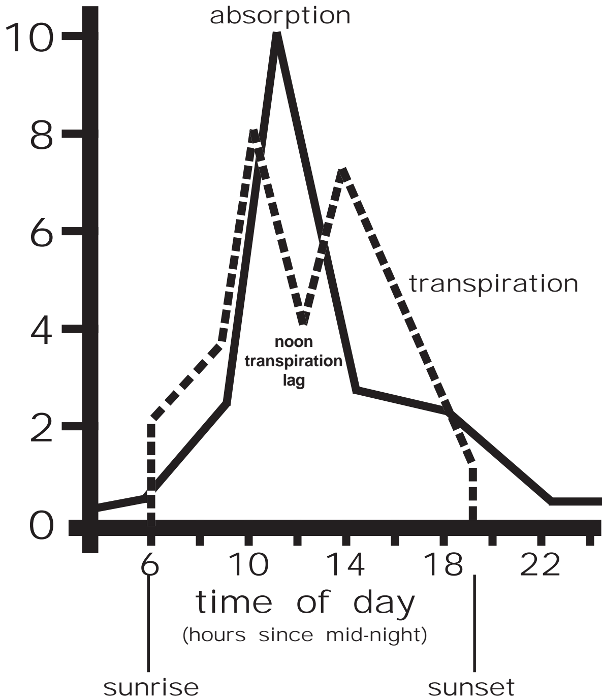
Figure 25: Root absorption and leaf transpiration within a tree and relative amount of water being moved by each process. Note transpiration in leaves begins just before sunrise, is slowed at mid-day, and stops just before sunset. Root absorption continues through the night.
