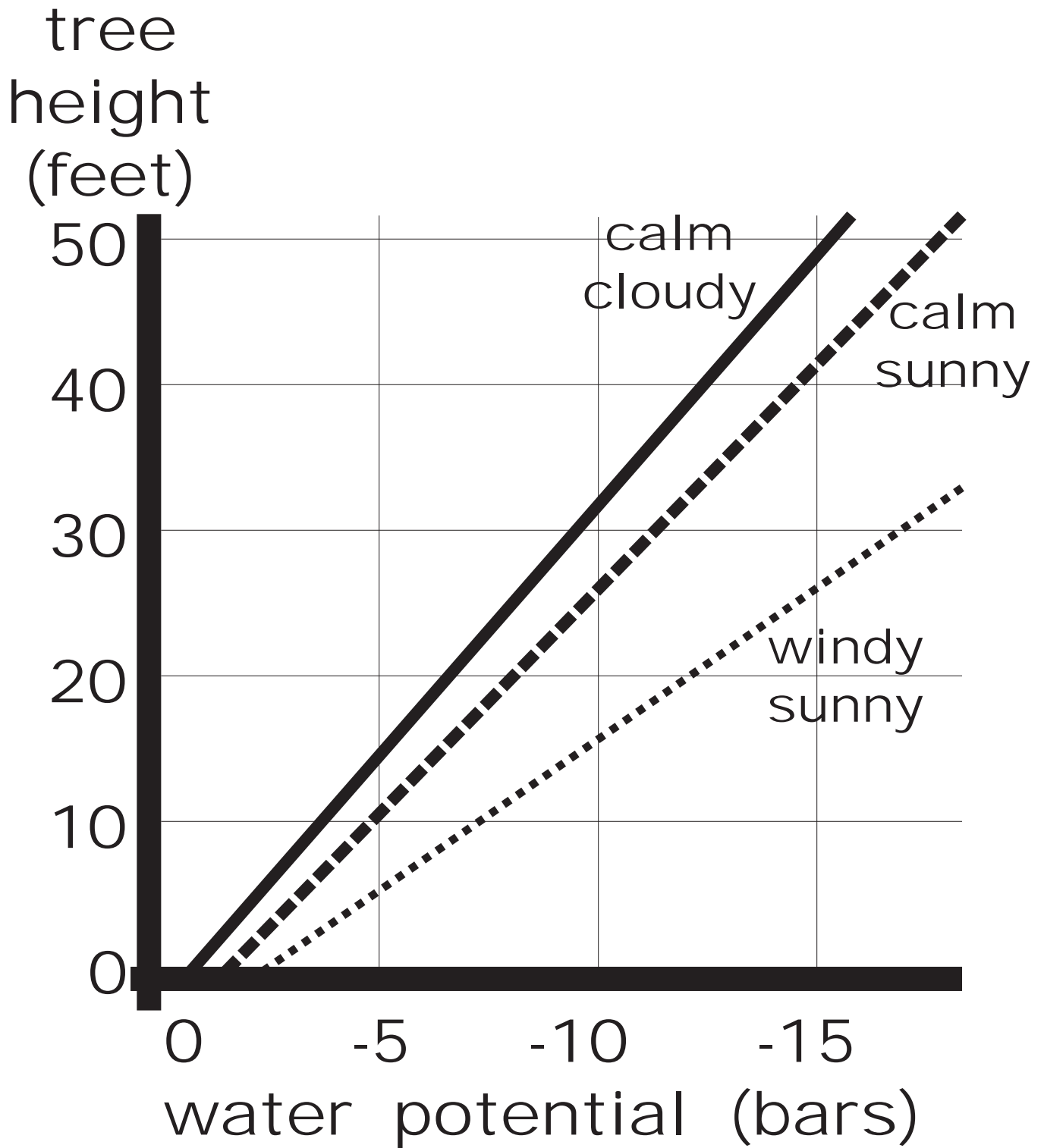
Figure 34: Mid-season water potential values at various tree heights under three site conditions: calm wind and cloudy; calm wind and sunny; and, windy and sunny. (derived from Hellkvist et. al. 1974)
