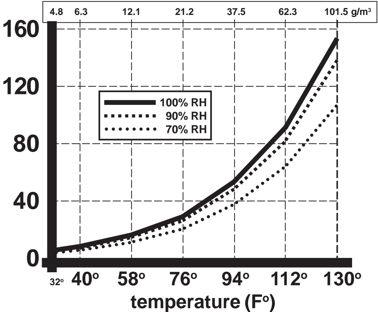
Figure 9: Saturated vapor pressure of water in atmosphere (100% relative humidity), the most water vapor normally found in air above liquid water. Also shown are 90% and 70% relative humidity (RH). The box over the graph contains the actual amount of water (vapor density in grams per cubic meter) in air for each temperature. (value approximations derived from Tabata, 1973)
