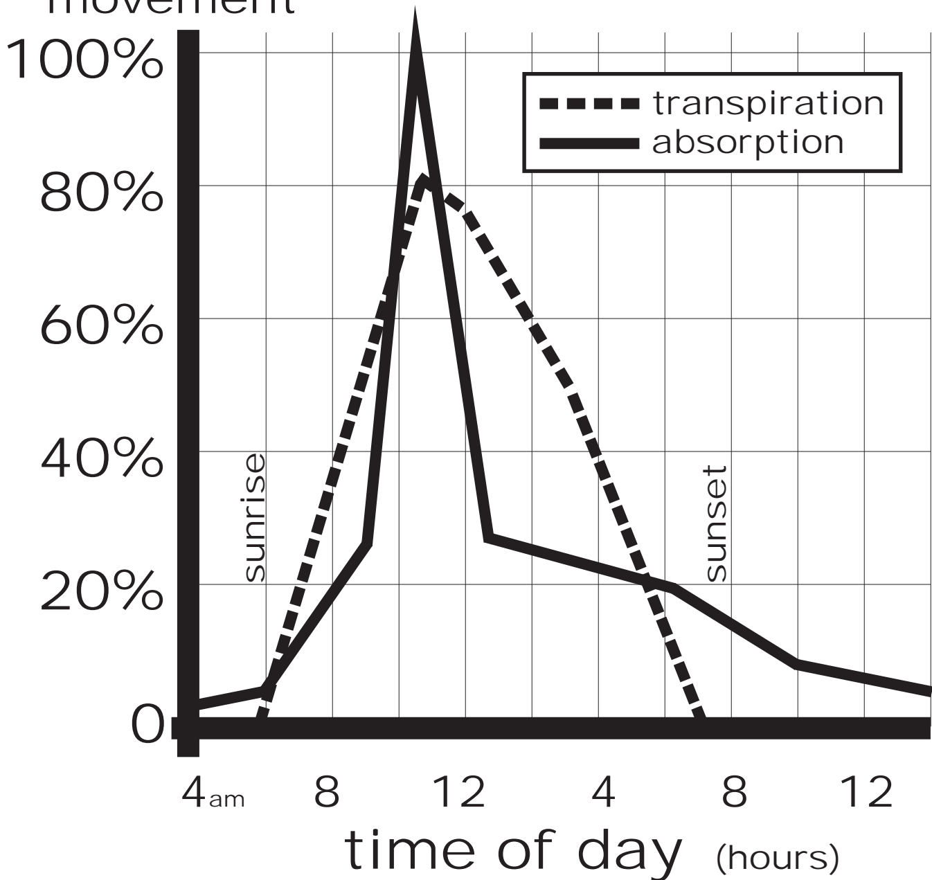
Figure 26: Example of relative ratio of water movement from transpiration and root absorption within a tree over a growing season day under field capacity soil water conditions with no noon transpiration lag. (derived from Waring & Schlesinger, 1985)
