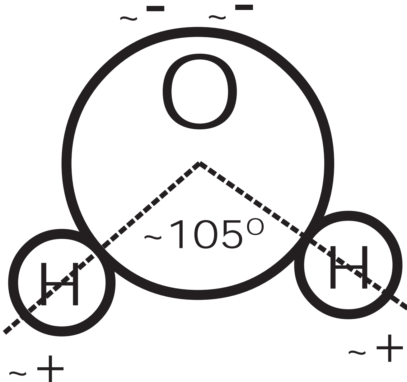
Figure 5: Diagram of water molecule with oxygen (O) and two hydrogen (H) atoms. Hydrogen atoms are always separated by \sim 105^\circ as they glide over the oxygen perimeter, never on opposite sides. Oxygen draws electrons away from hydrogens generating a polar molecule with partial negative charges ( \sim - ) on the oxygen side and partial positive charges ( \sim + ) on the hydrogen side.
